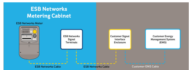
Figure 1: Customer signals equipment layout Signal Information
